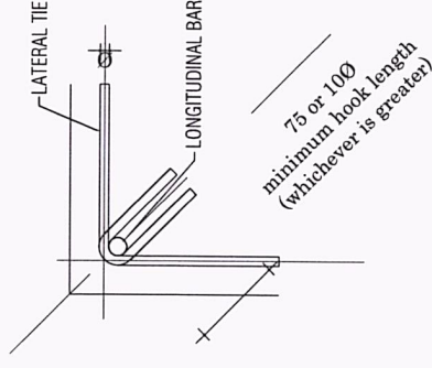
DETAILS A-135° HOOK DETAIL FOR STIRRUPS & TIES
