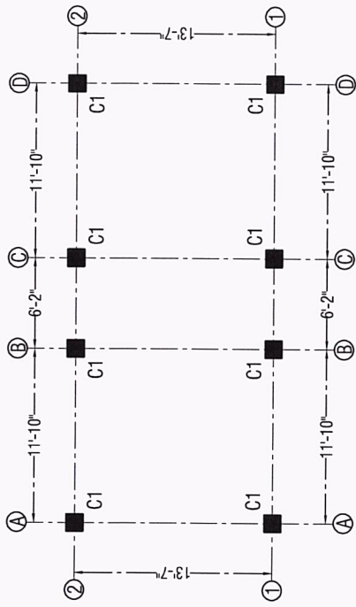
LAYOUT OF COLUMN PLAN
