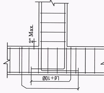
TYPICAL BAR DETAIL AT CORNER
